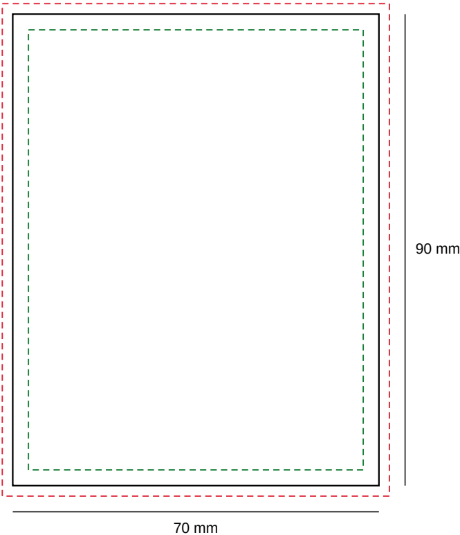
Front sticker: 70 × 90 mm trim · 2 mm bleed · 3 mm safe
