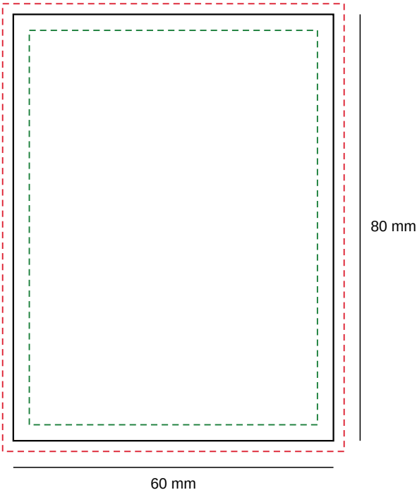
Back sticker (legal panel): 60 × 80 mm trim · 2 mm bleed · 3 mm safe
